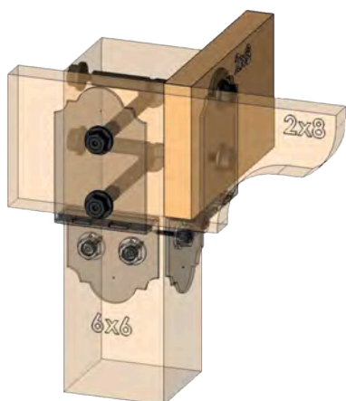
Bolt Offset
