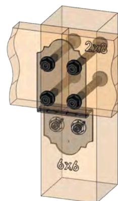
Coupler
