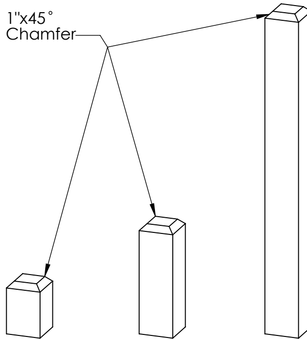
6x6x8 Post (cut all wood from 1 post)
