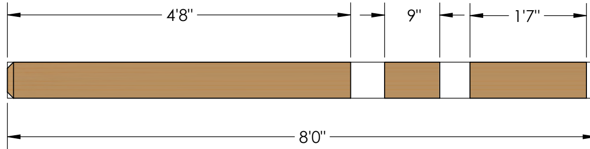
6x6x8 Post (cut all wood from 1 post)
